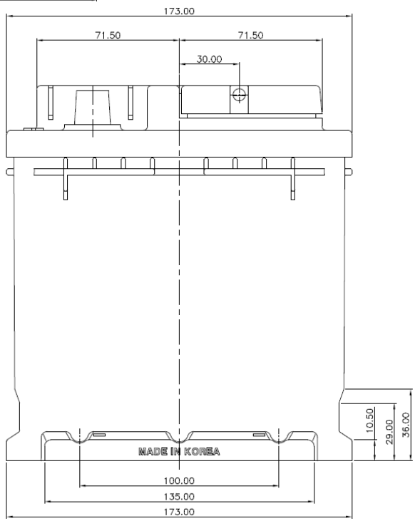
POSITIVE TERMINAL
